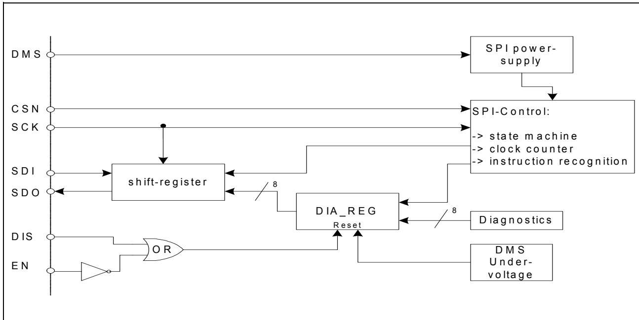
Figure 6 SPI block-diagram
