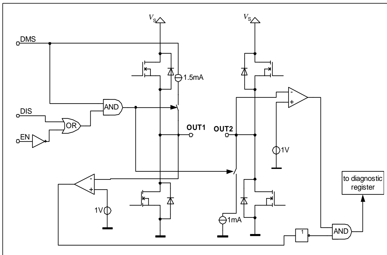
Figure 9 Functional block diagram of open-load detection
