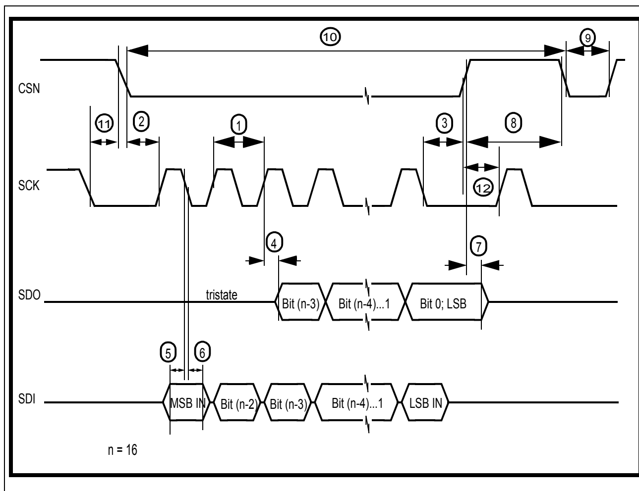
Figure 13 SPI-timing
